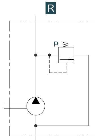
Emniyet Valfi Relief Valve
